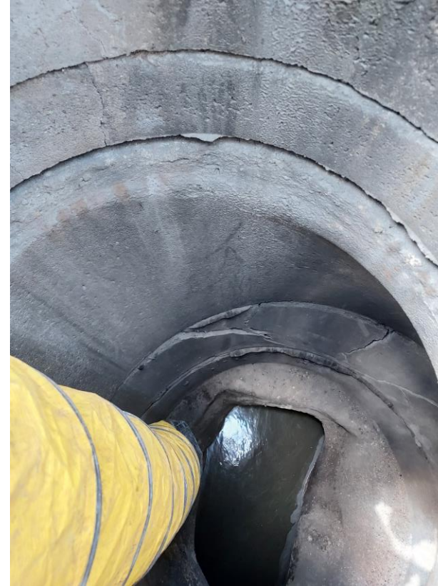
Fig. 2 – Failed manhole
